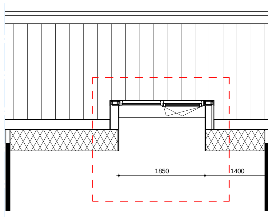
9312400_dakkapel-1850
